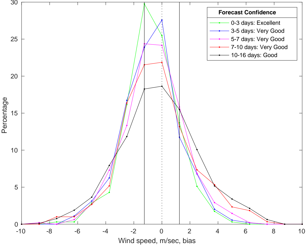
NDBC 42040 vs GFS Winds Bias Histogram: 05-Jul-2025
