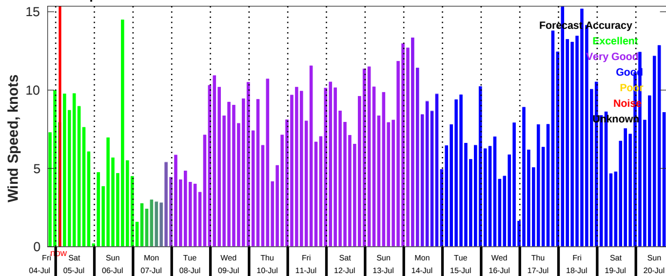
GFS Wind Speed Forecast for NDBC 42040 from 04-Jul-2025 19:00:00 to 20-Jul-2025 19:00:00
