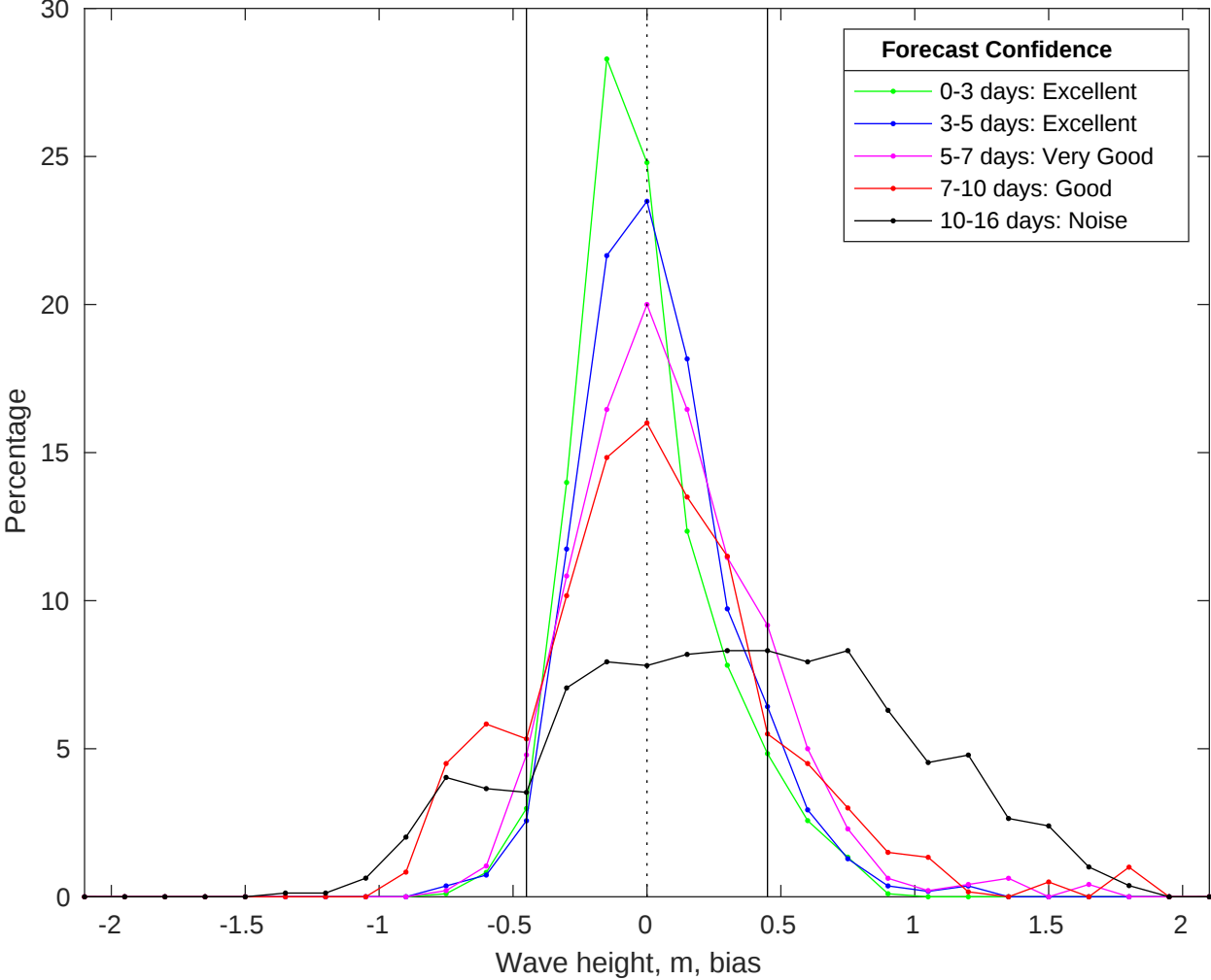
NDBC 46011 vs GFS Waves Bias Histogram: 05-Jul-2025
