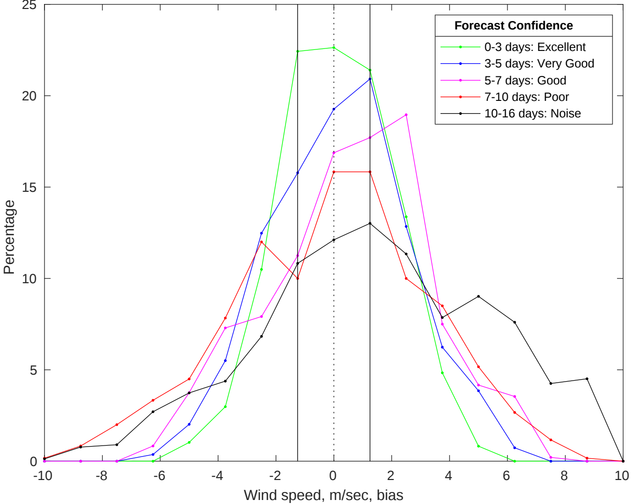
NDBC 46011 vs GFS Winds Bias Histogram: 05-Jul-2025
