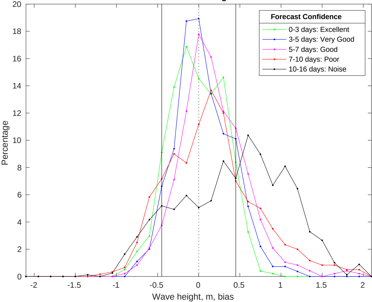
NDBC 46028 vs GFS Waves Bias Histogram: 05-Jul-2025
