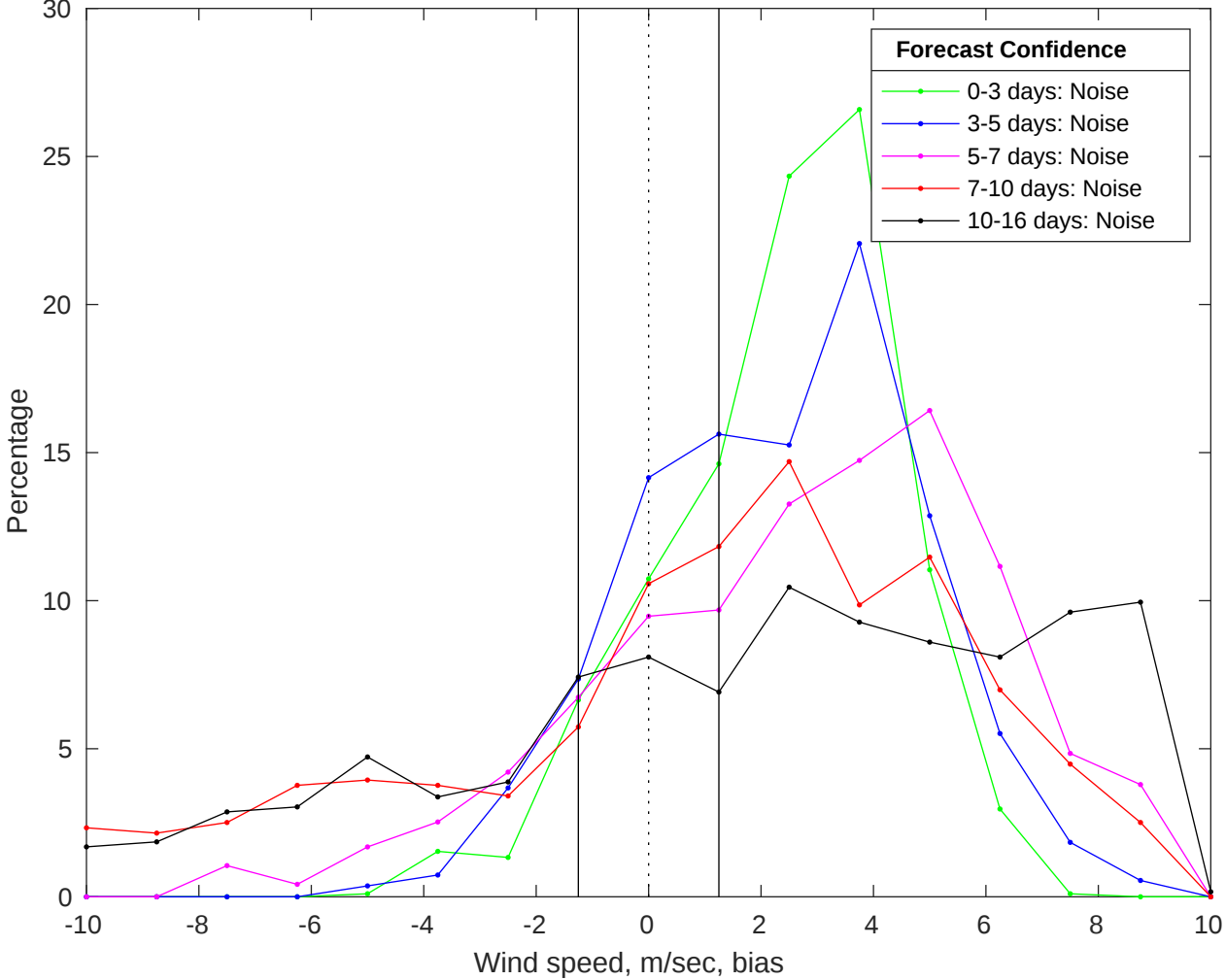
NDBC 46028 vs GFS Winds Bias Histogram: 05-Jul-2025
