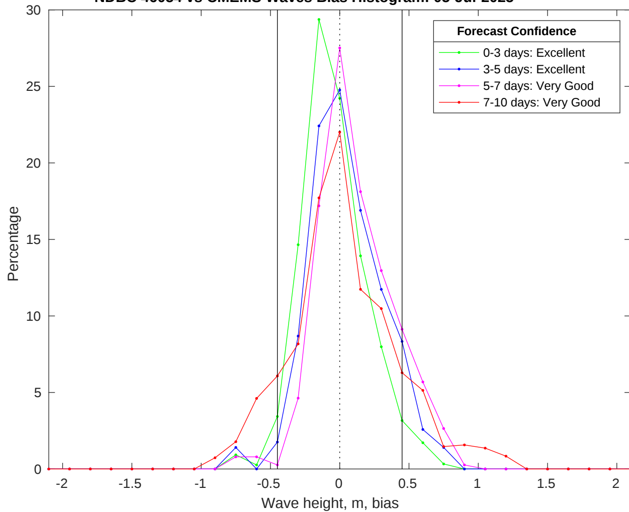
NDBC 46054 vs CMEMS Waves Bias Histogram: 05-Jul-2025
