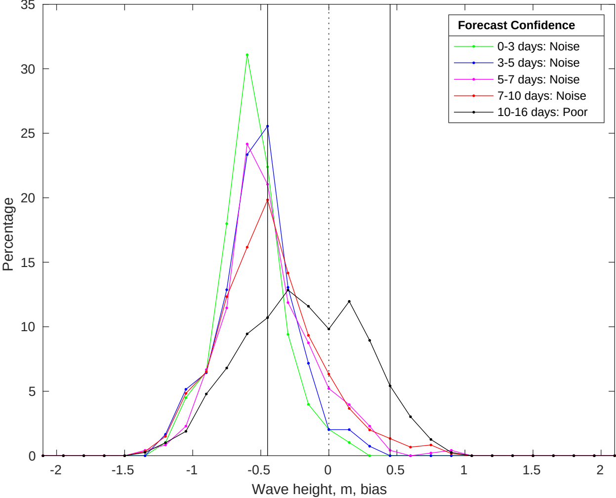
NDBC 46054 vs GFS Waves Bias Histogram: 05-Jul-2025
