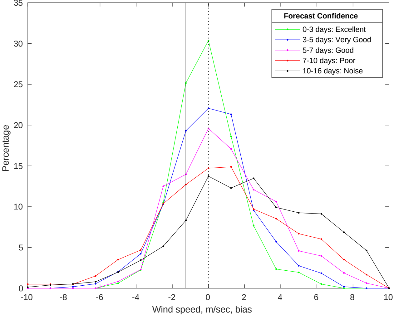
NDBC 46054 vs GFS Winds Bias Histogram: 05-Jul-2025
