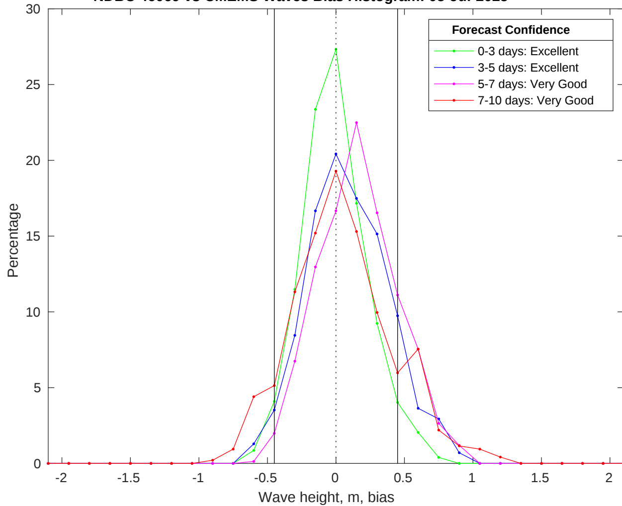
NDBC 46069 vs CMEMS Waves Bias Histogram: 05-Jul-2025
