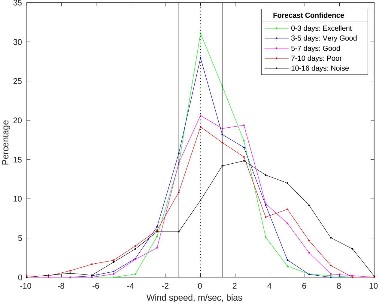
NDBC 46069 vs GFS Winds Bias Histogram: 05-Jul-2025
