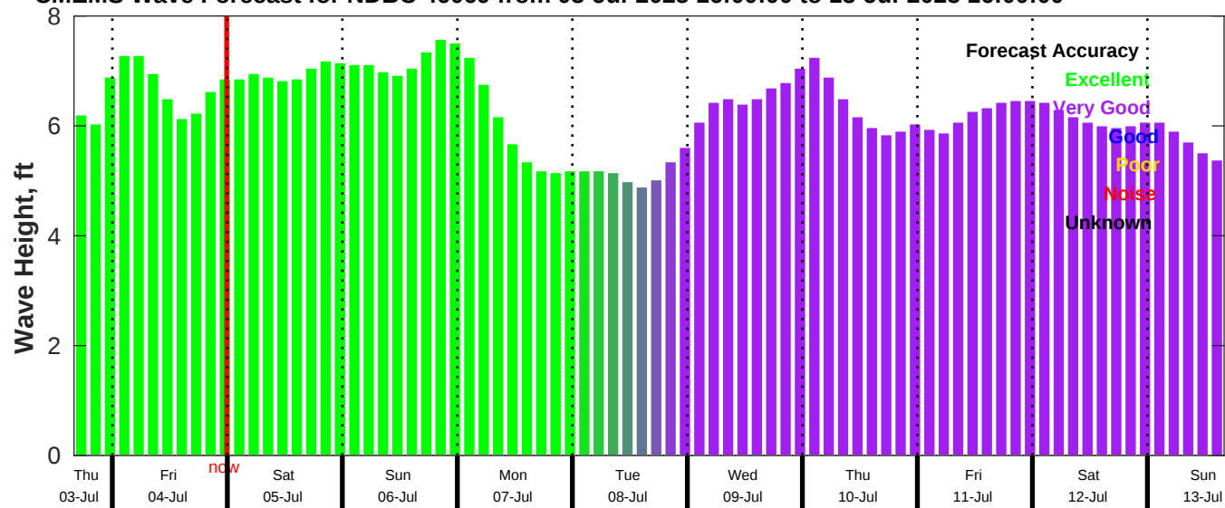
CMEMS Wave Forecast for NDBC 46069 from 03-Jul-2025 16:00:00 to 13-Jul-2025 16:00:00
