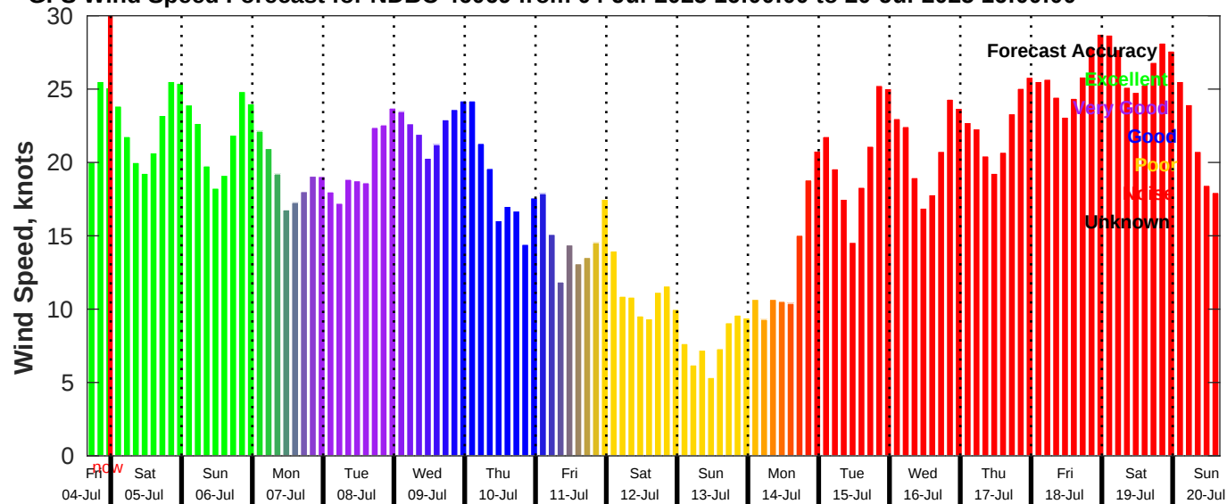
GFS Wind Speed Forecast for NDBC 46069 from 04-Jul-2025 16:00:00 to 20-Jul-2025 16:00:00
