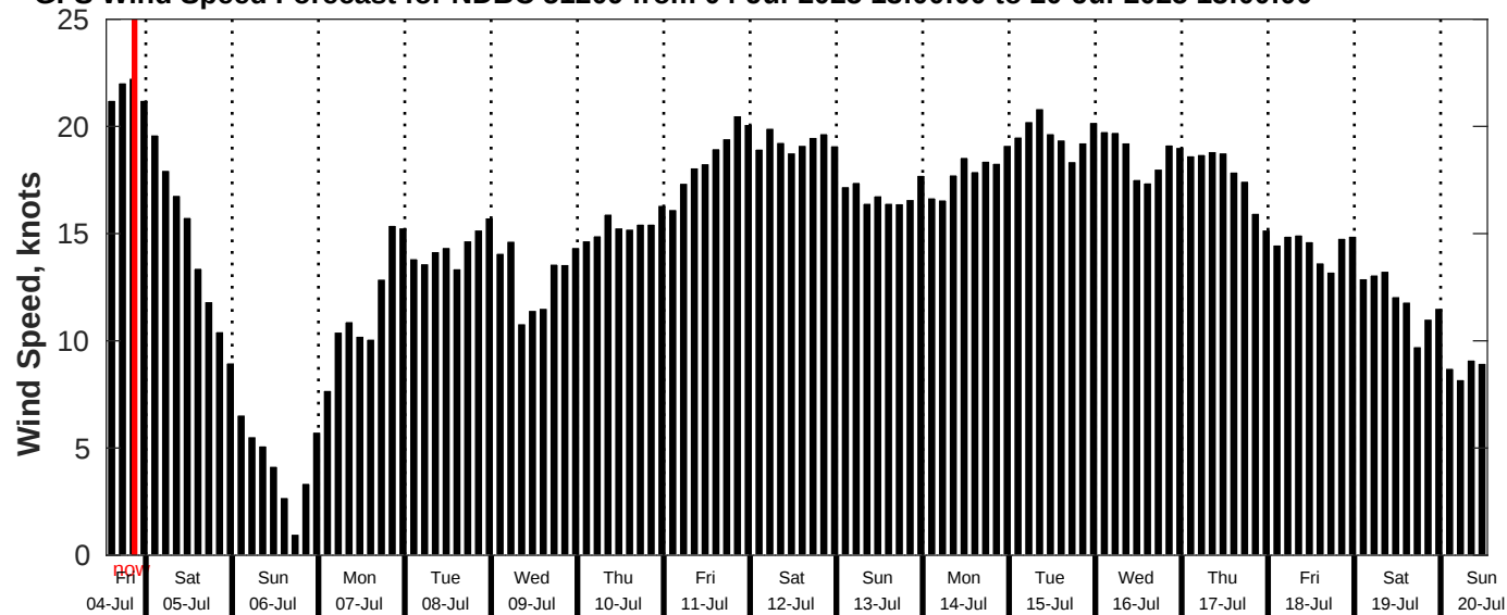
GFS Wind Speed Forecast for NDBC 51209 from 04-Jul-2025 13:00:00 to 20-Jul-2025 13:00:00
