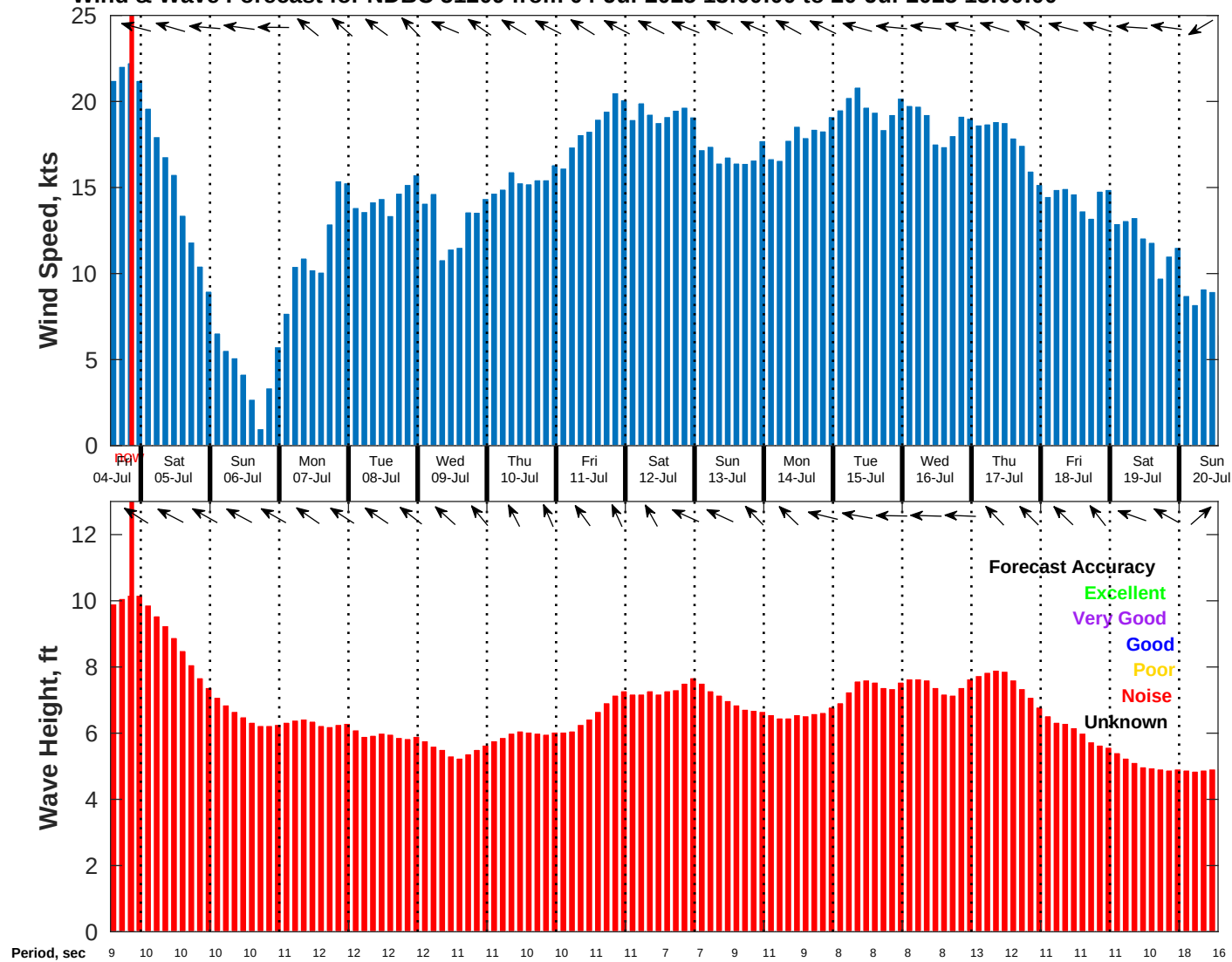
Wind & Wave Forecast for NDBC 51209 from 04-Jul-2025 13:00:00 to 20-Jul-2025 13:00:00
