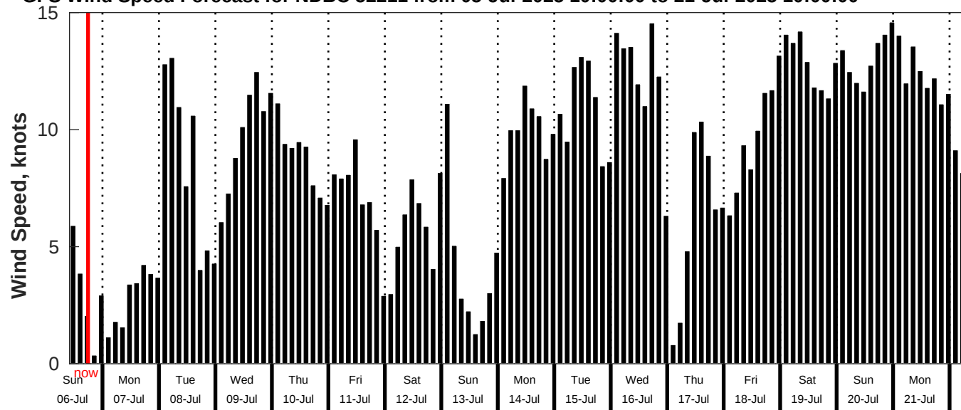
GFS Wind Speed Forecast for NDBC 52211 from 05-Jul-2025 10:00:00 to 21-Jul-2025 10:00:00
