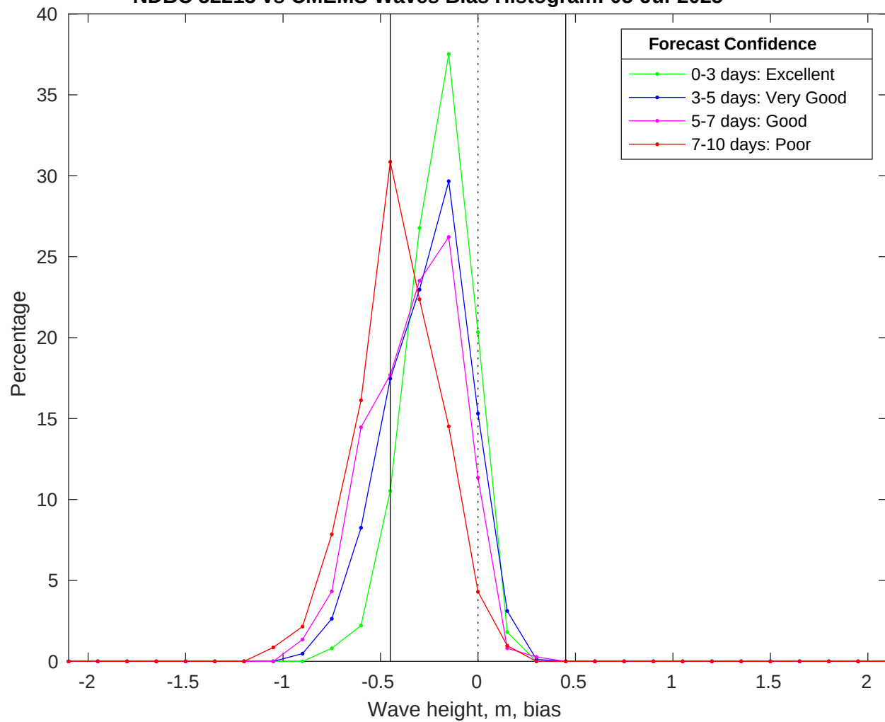
NDBC 52213 vs CMEMS Waves Bias Histogram: 05-Jul-2025
