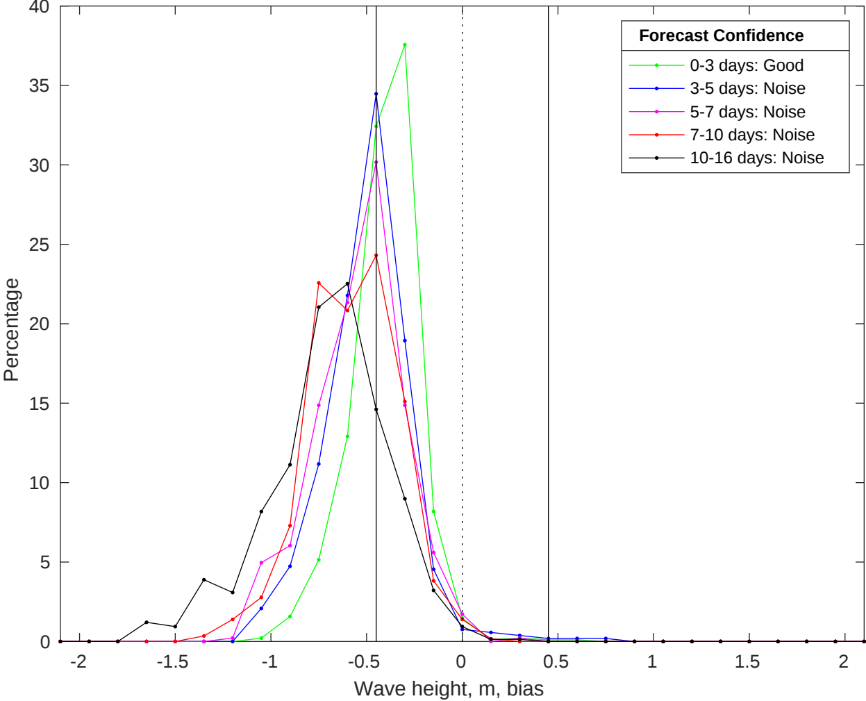
NDBC 52213 vs GFS Waves Bias Histogram: 05-Jul-2025
