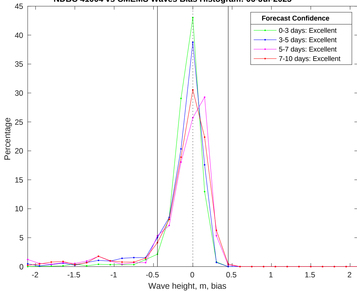
NDBC 41004 vs CMEMS Waves Bias Histogram: 06-Jul-2025
