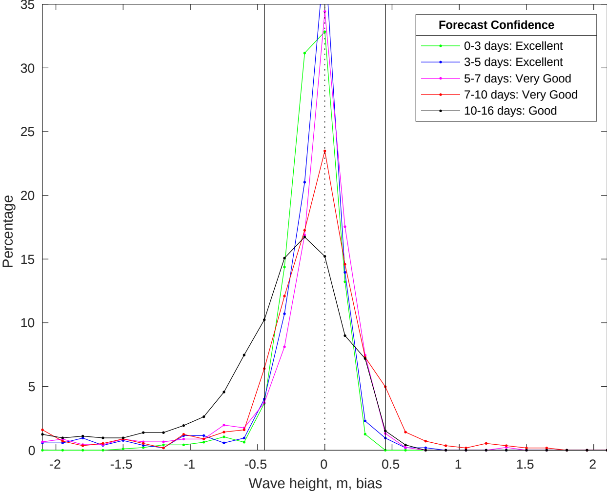
NDBC 41004 vs GFS Waves Bias Histogram: 06-Jul-2025
