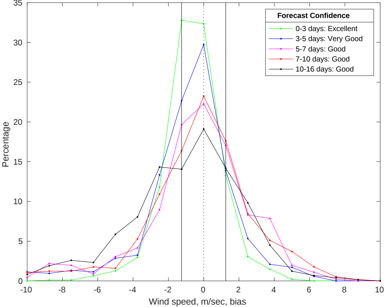
NDBC 41004 vs GFS Winds Bias Histogram: 06-Jul-2025
