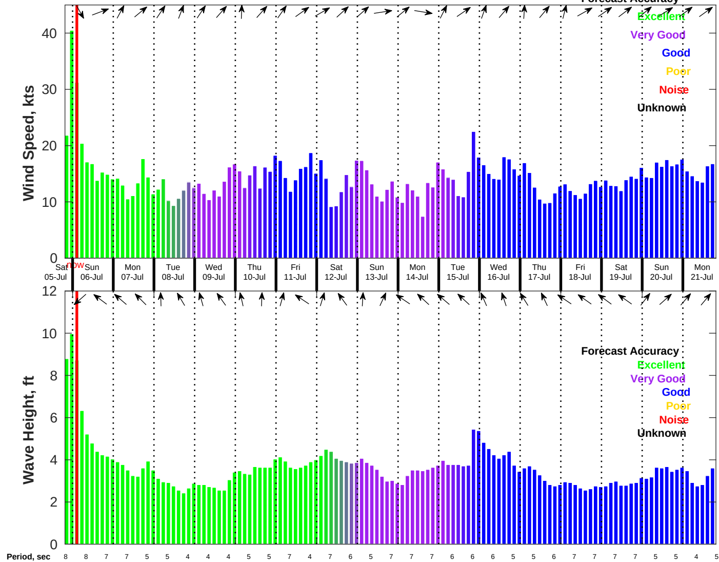
Wind & Wave Forecast for NDBC 41004 from 05-Jul-2025 19:00:00 to 21-Jul-2025 19:00:00
