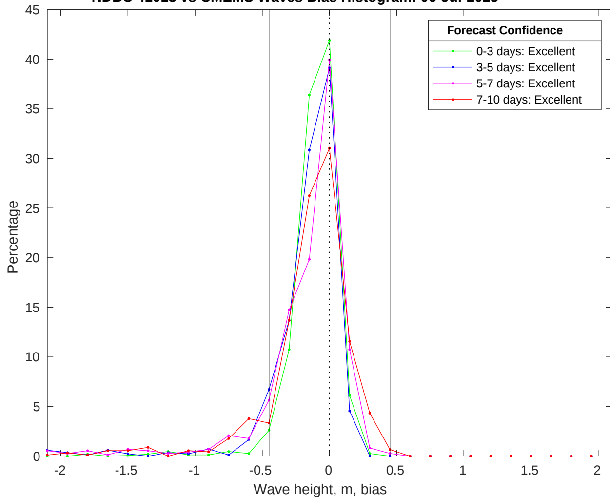
NDBC 41013 vs CMEMS Waves Bias Histogram: 06-Jul-2025
