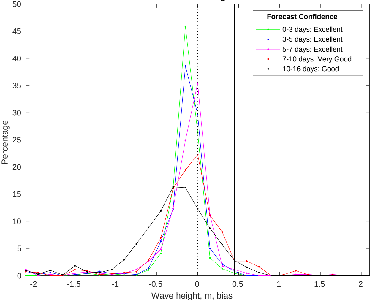
NDBC 41013 vs GFS Waves Bias Histogram: 06-Jul-2025
