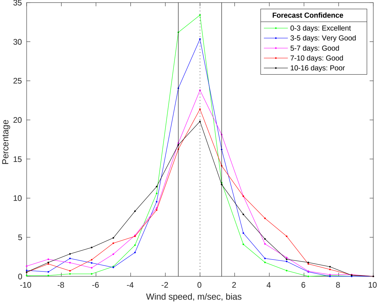
NDBC 41013 vs GFS Winds Bias Histogram: 06-Jul-2025
