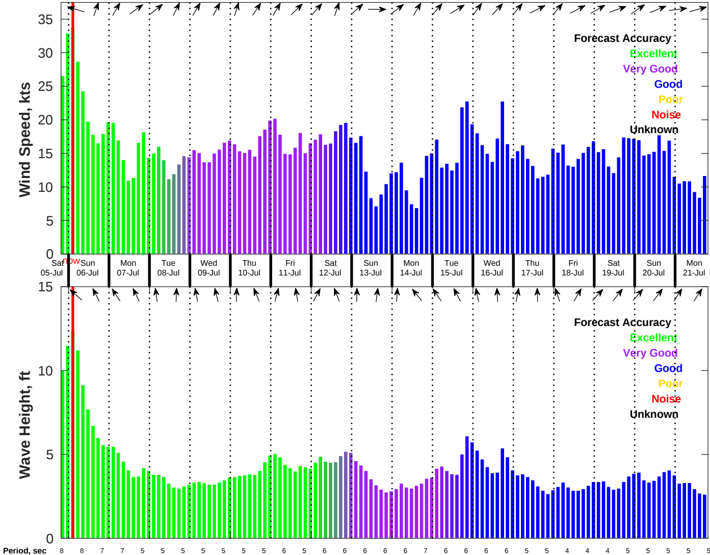
Wind & Wave Forecast for NDBC 41013 from 05-Jul-2025 19:00:00 to 21-Jul-2025 19:00:00
