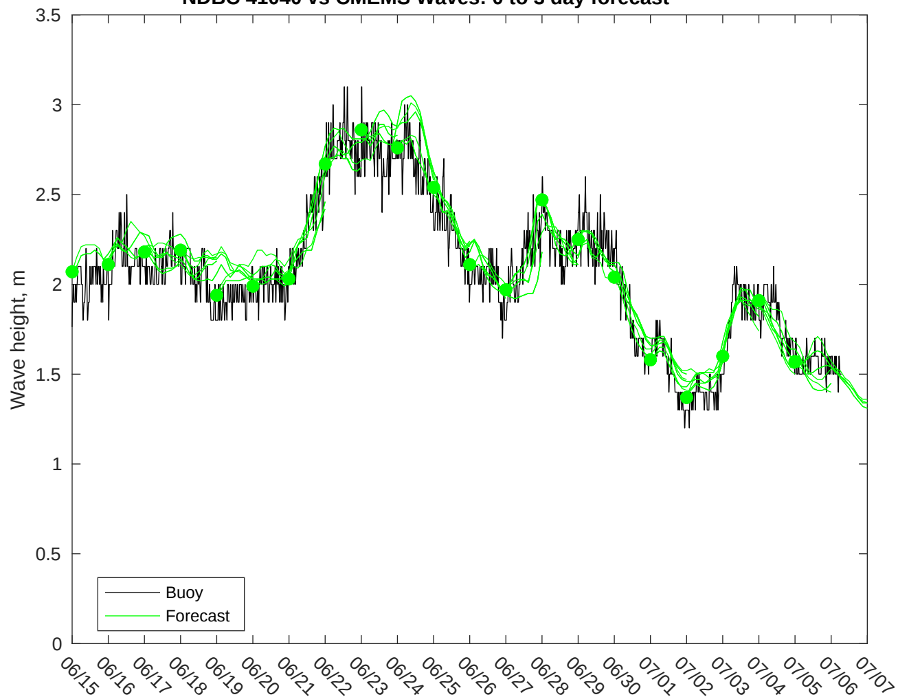
NDBC 41040 vs CMEMS Waves: 0 to 3 day forecast
