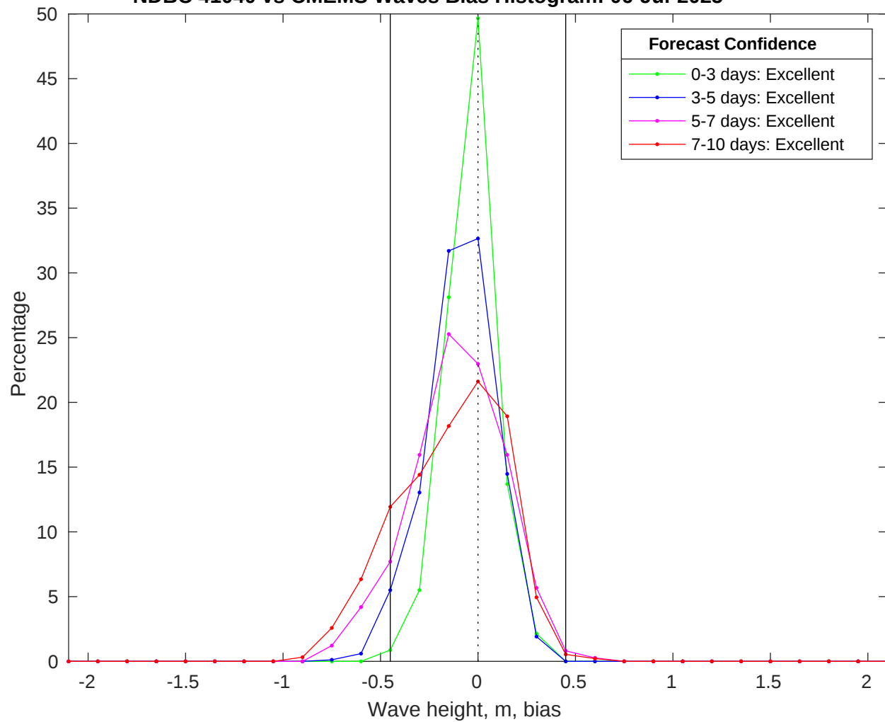
NDBC 41040 vs CMEMS Waves Bias Histogram: 06-Jul-2025
