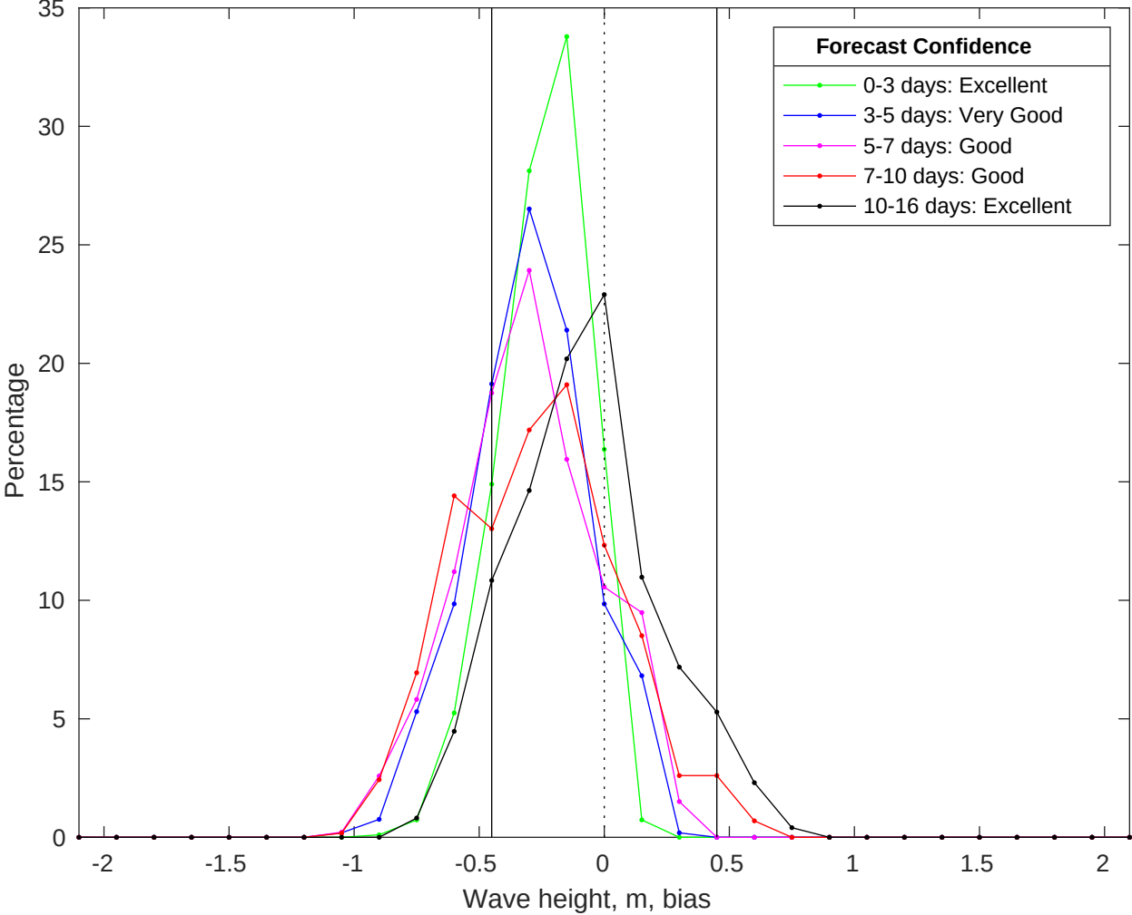
NDBC 41040 vs GFS Waves Bias Histogram: 06-Jul-2025
