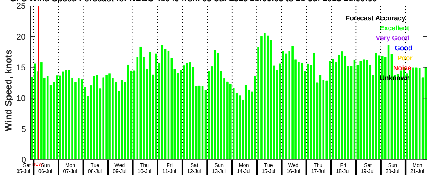
GFS Wind Speed Forecast for NDBC 41040 from 05-Jul-2025 21:00:00 to 21-Jul-2025 21:00:00
