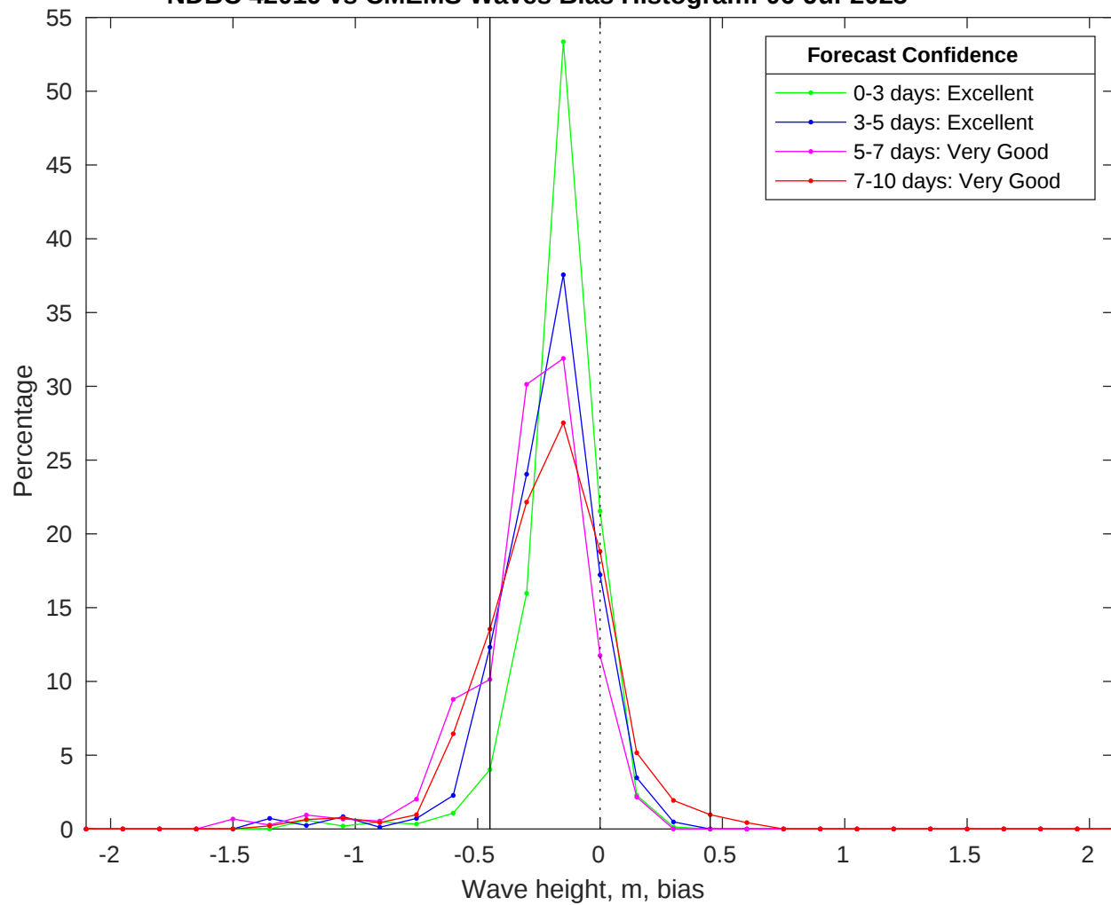
NDBC 42019 vs CMEMS Waves Bias Histogram: 06-Jul-2025
