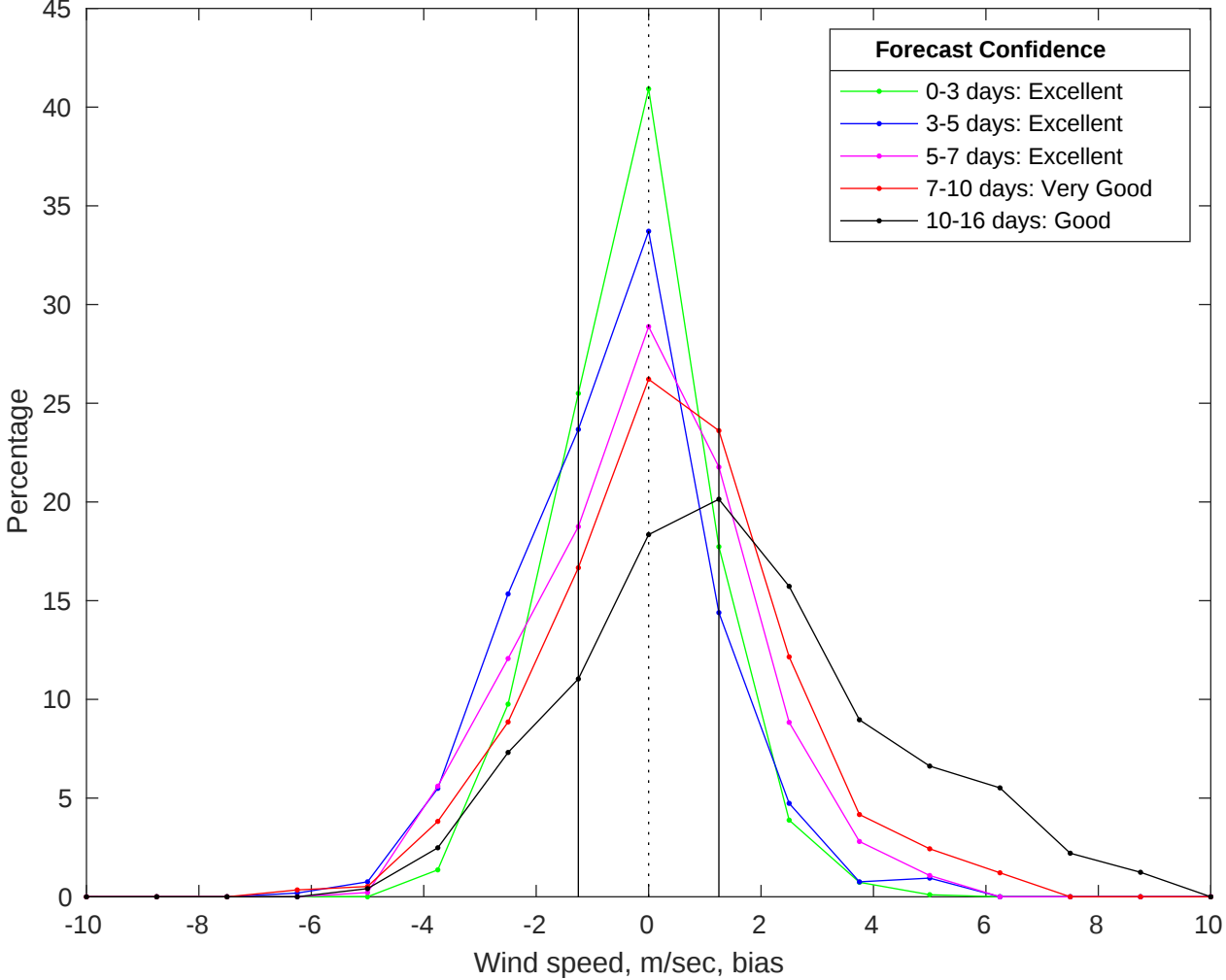
NDBC 42019 vs GFS Winds Bias Histogram: 06-Jul-2025
