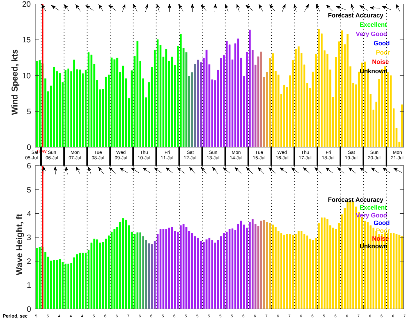
Wind & Wave Forecast for NDBC 42019 from 05-Jul-2025 18:00:00 to 21-Jul-2025 18:00:00
