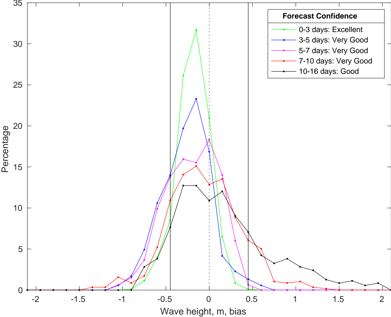
NDBC 42020 vs GFS Waves Bias Histogram: 06-Jul-2025
