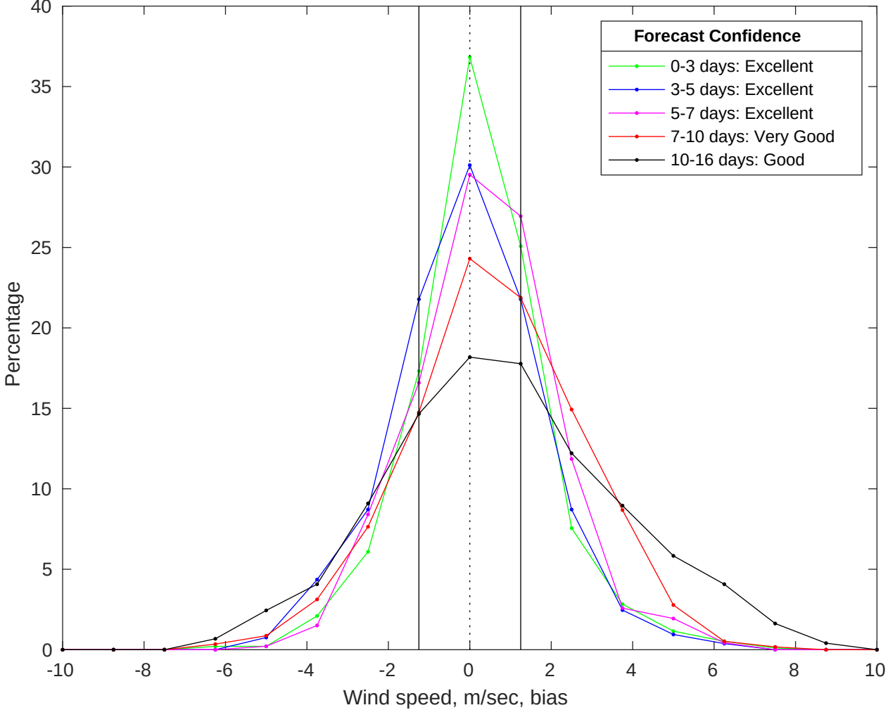
NDBC 42020 vs GFS Winds Bias Histogram: 06-Jul-2025
