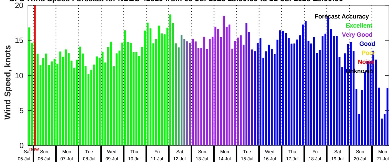
GFS Wind Speed Forecast for NDBC 42020 from 05-Jul-2025 18:00:00 to 21-Jul-2025 18:00:00
