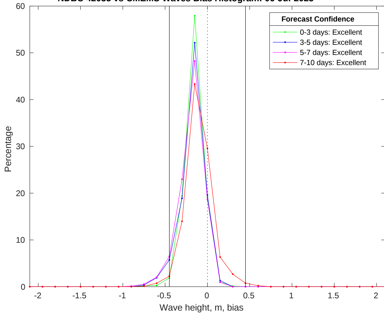
NDBC 42035 vs CMEMS Waves Bias Histogram: 06-Jul-2025
