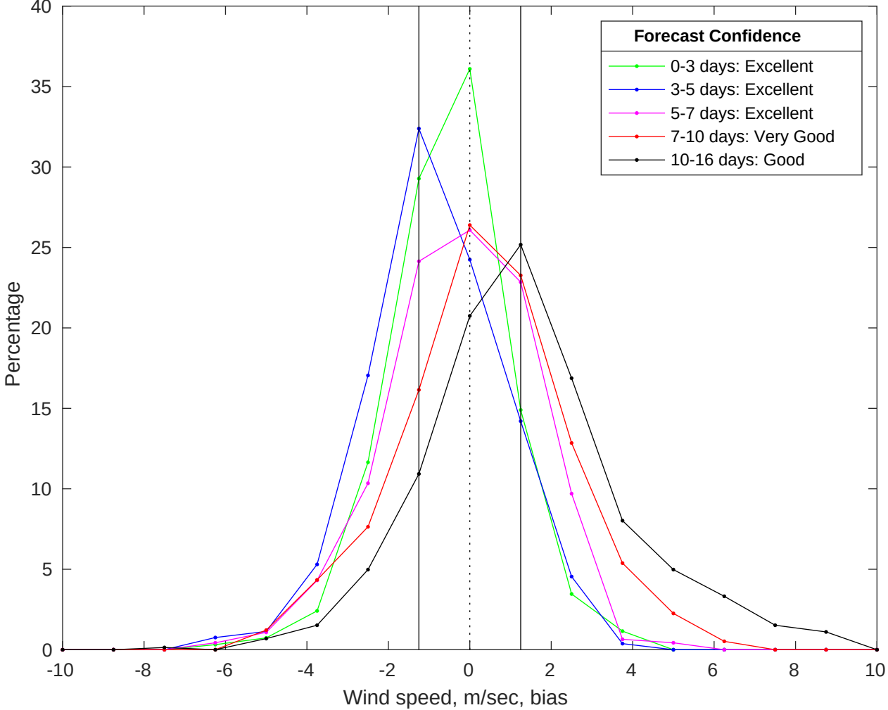
NDBC 42035 vs GFS Winds Bias Histogram: 06-Jul-2025
