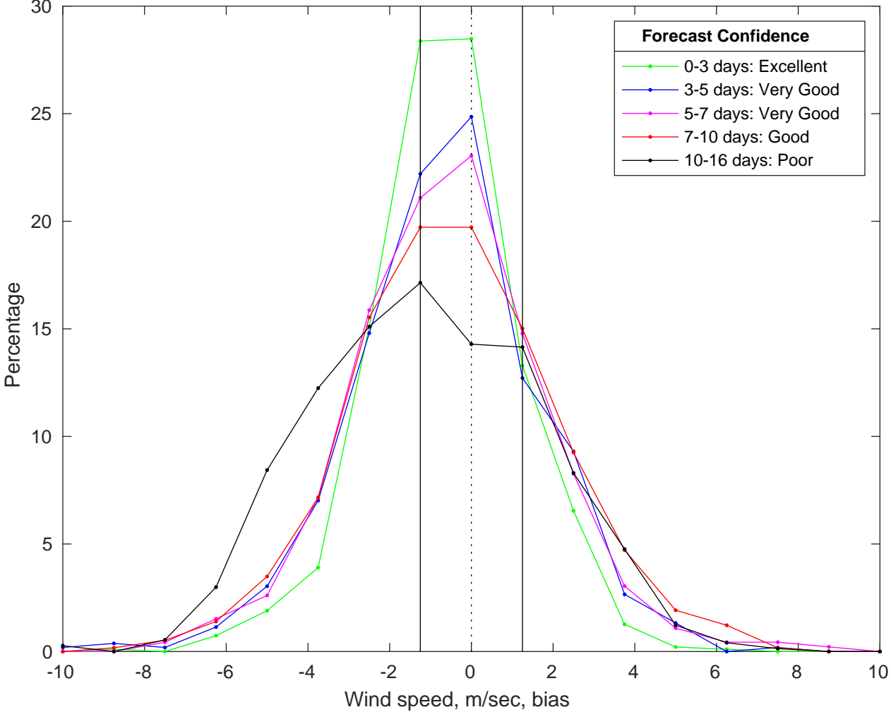
NDBC 42036 vs GFS Winds Bias Histogram: 06-Jul-2025
