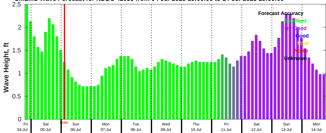
CMEMS Wave Forecast for NDBC 42036 from 04-Jul-2025 19:00:00 to 14-Jul-2025 19:00:00
