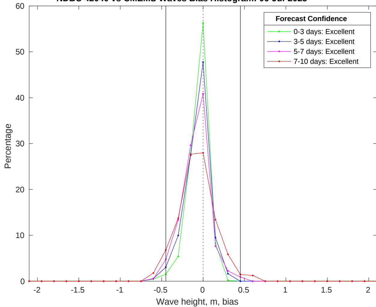
NDBC 42040 vs CMEMS Waves Bias Histogram: 06-Jul-2025
