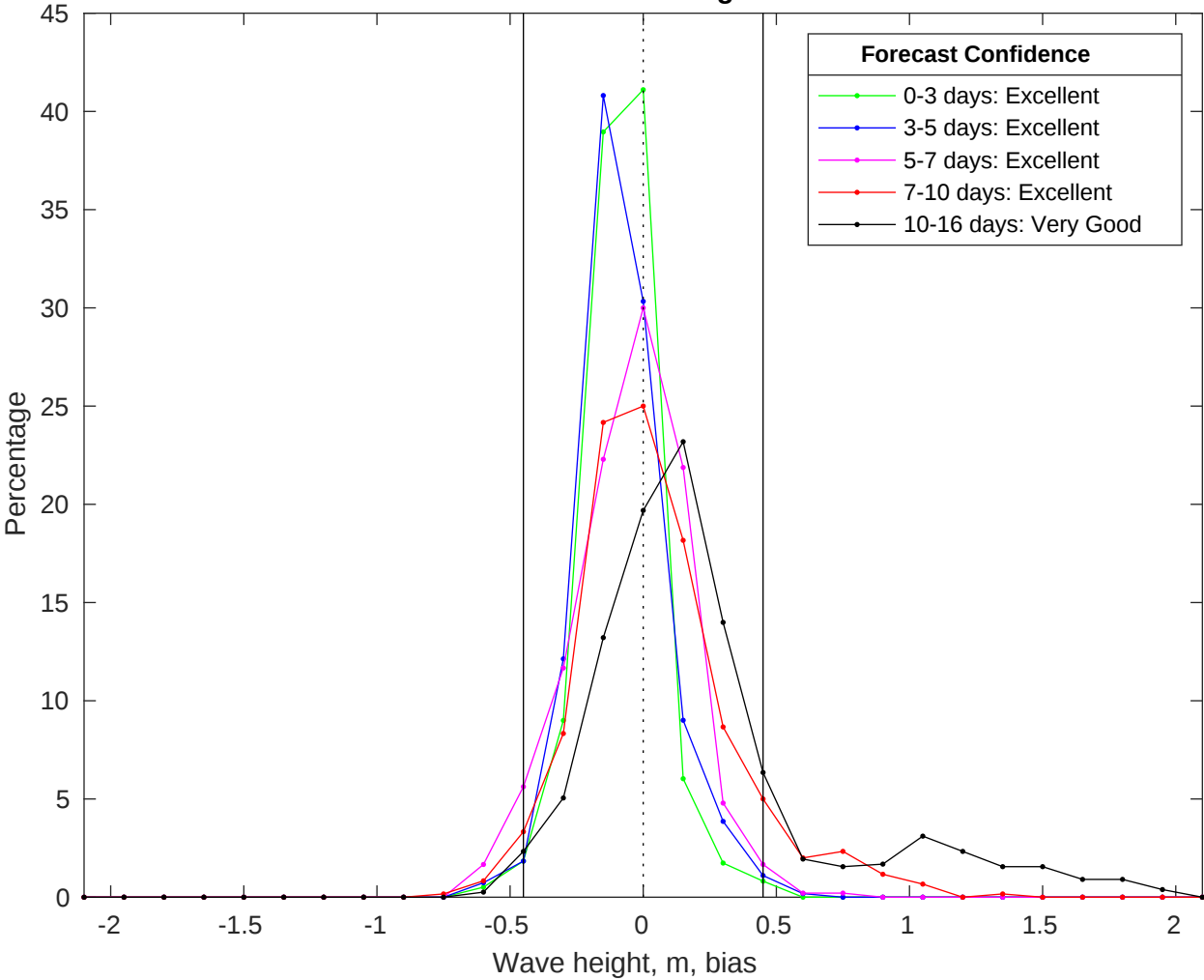
NDBC 42040 vs GFS Waves Bias Histogram: 06-Jul-2025
