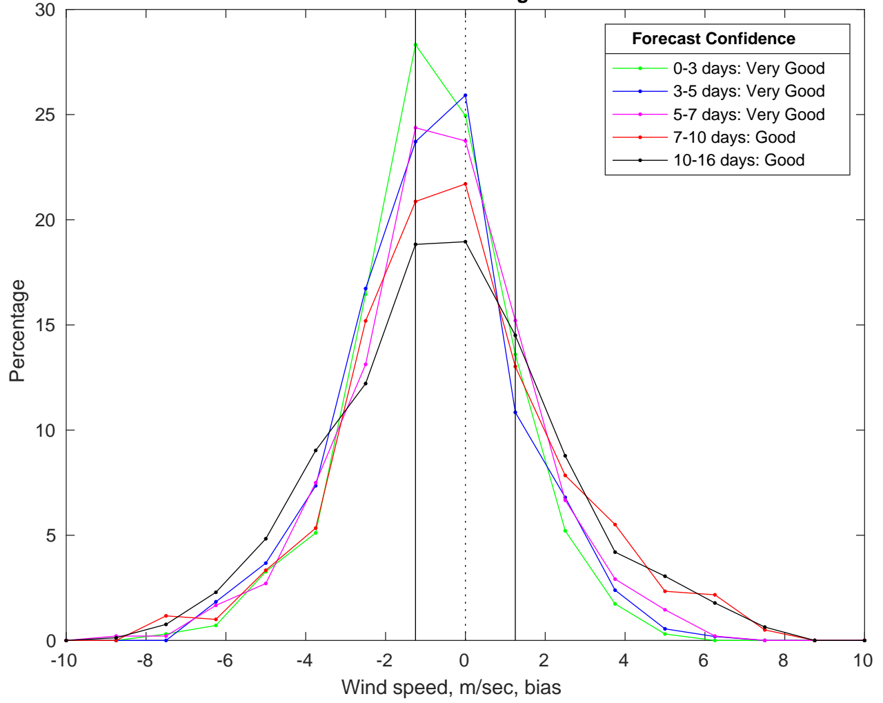
NDBC 42040 vs GFS Winds Bias Histogram: 06-Jul-2025
