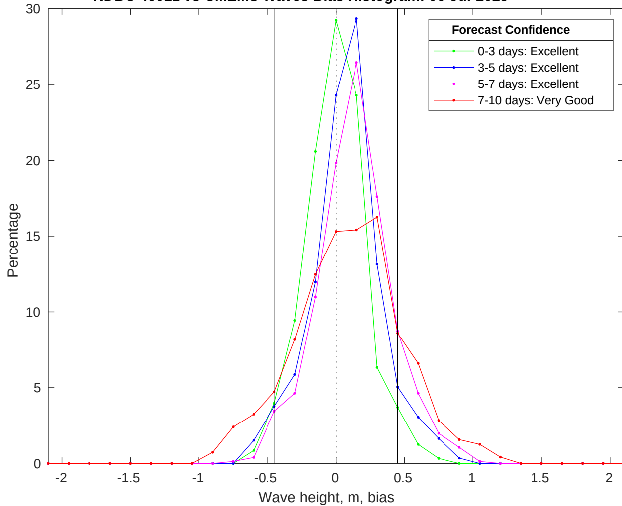
NDBC 46011 vs CMEMS Waves Bias Histogram: 06-Jul-2025
