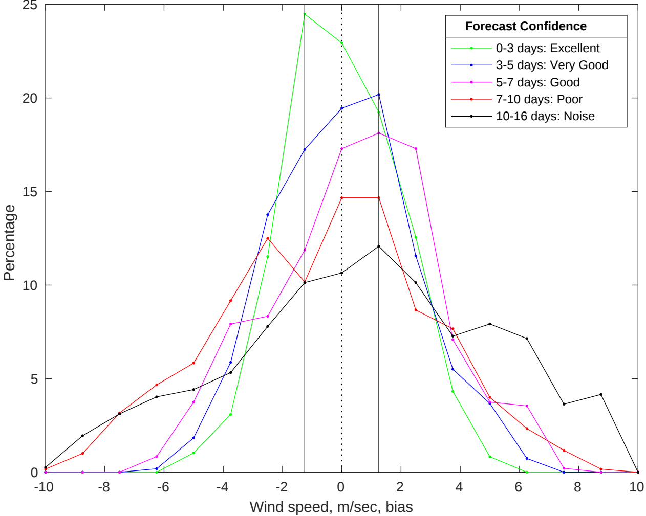
NDBC 46011 vs GFS Winds Bias Histogram: 06-Jul-2025
