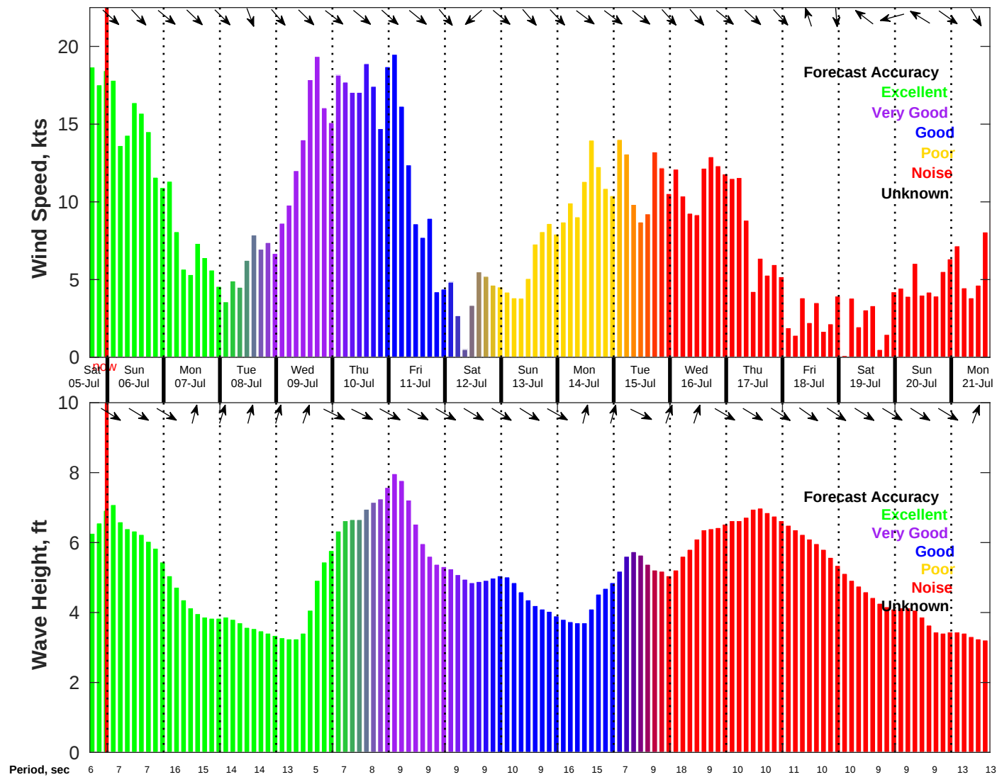
Wind & Wave Forecast for NDBC 46011 from 05-Jul-2025 16:00:00 to 21-Jul-2025 16:00:00
