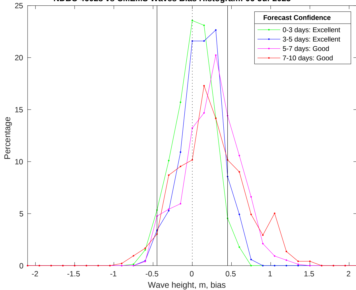
NDBC 46028 vs CMEMS Waves Bias Histogram: 06-Jul-2025
