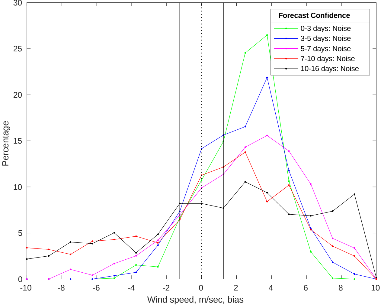
NDBC 46028 vs GFS Winds Bias Histogram: 06-Jul-2025
