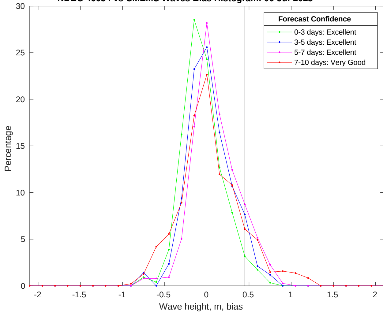
NDBC 46054 vs CMEMS Waves Bias Histogram: 06-Jul-2025
