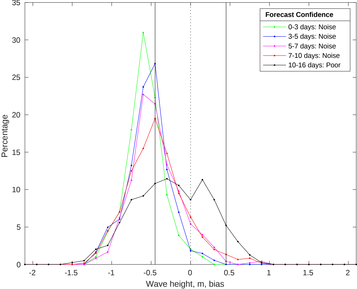
NDBC 46054 vs GFS Waves Bias Histogram: 06-Jul-2025
